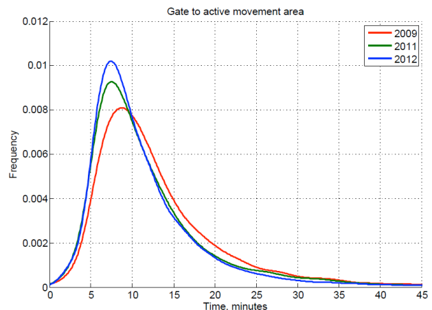
Figure 12. Distribution of time spent taxiing from gate to stop.
