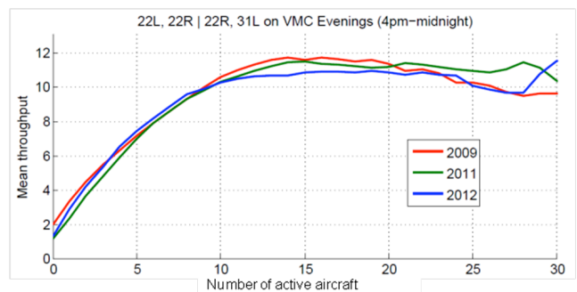
Figure 4. Runway throughput saturation in the 22L, 22R | 22R, 31L configuration, on good weather evenings.
